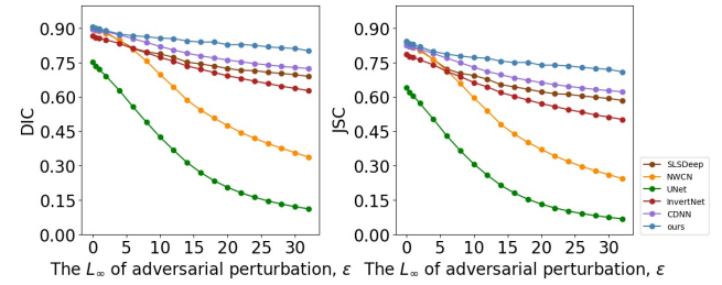
Figure 5: Comparison of quantitative results in terms of DIC and JSC on ISBI 2016 skin lesion segmentation dataset.
