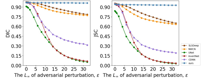
Figure 4: Comparison of quantitative results in terms of DIC and JSC on the JSRT lung segmentation dataset.
